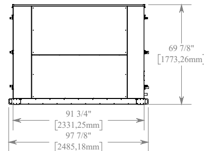
RIGHT VIEW
